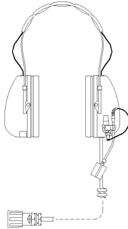
ISMIC 06/07 Intrinsic safe ear Defender Headset & Boom Microphone for use with 7403/0/02
