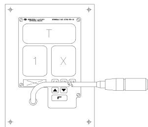
Ex 7451 Flush fit intrinsic safe remote keypad / gooseneck microphone for use with
