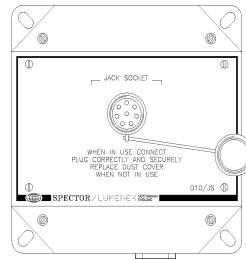
D10/JS Intrinsic Safe Jack Socket Box for use with ISMIC 06/07.
