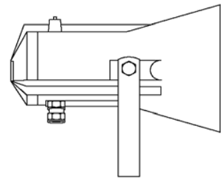
15 Watt Extension Loudspeaker
