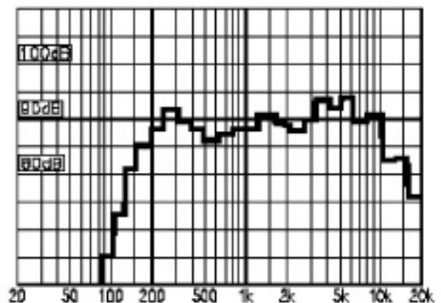
1W/1m 1/3 octave pink noise
